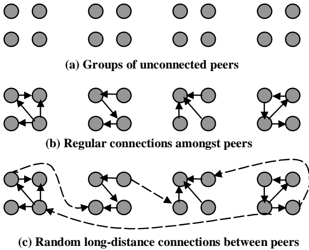
Figure 1: Creation of a P2P small-world network
