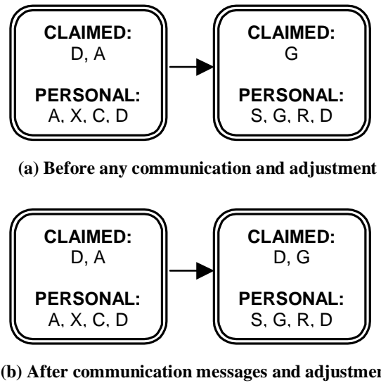
Figure 2: Procedure to escalate attributes (D in this case). Two peers that are linked (shown by arrow) are considered for the illustration.
